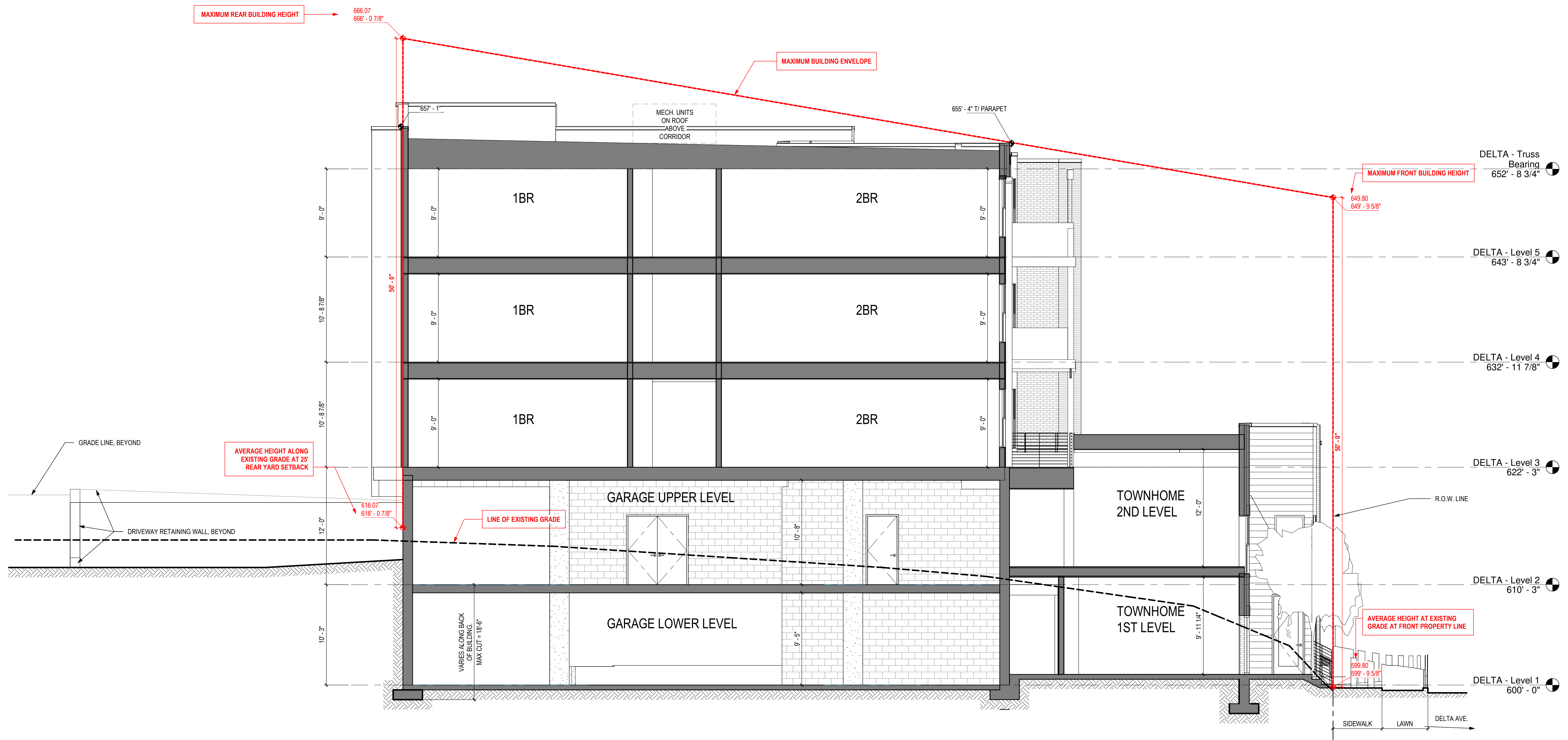
1 site section - zoning #6 SK4.6 3/16" = 1'-0"
